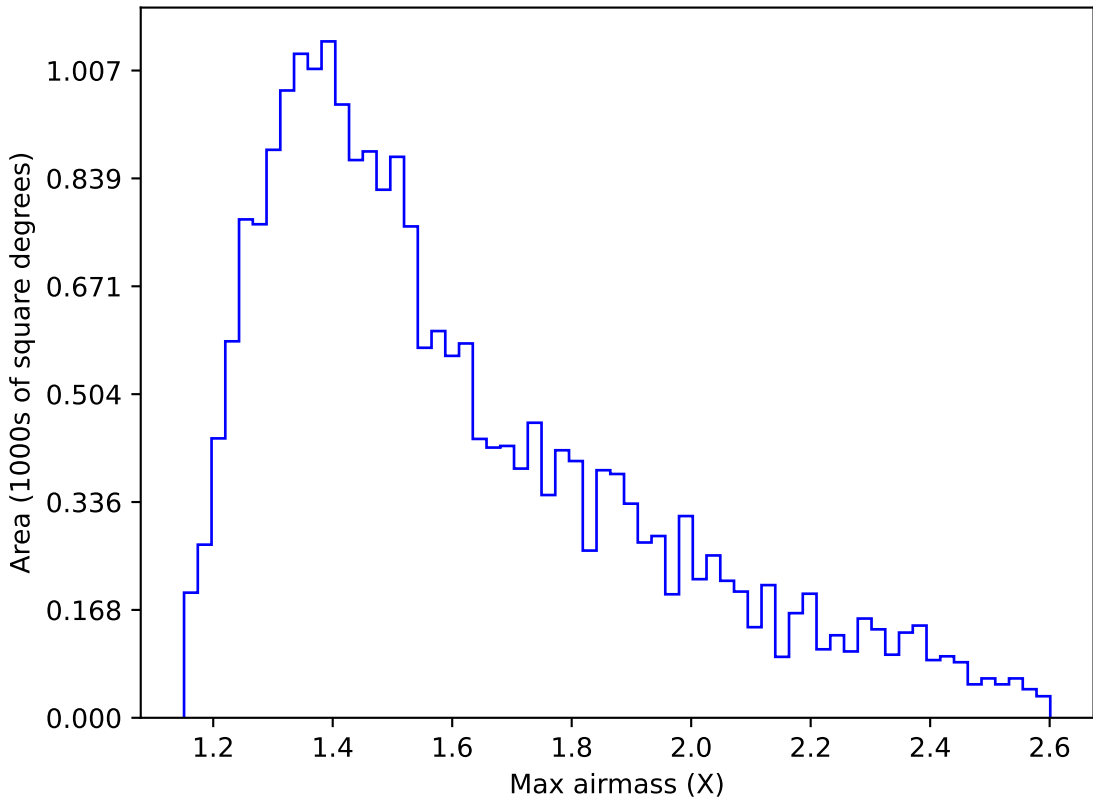
ddf_acor_sf10_lsf40_lsr20_v3.4_10yrs Yr 1 y band: Max airmass
