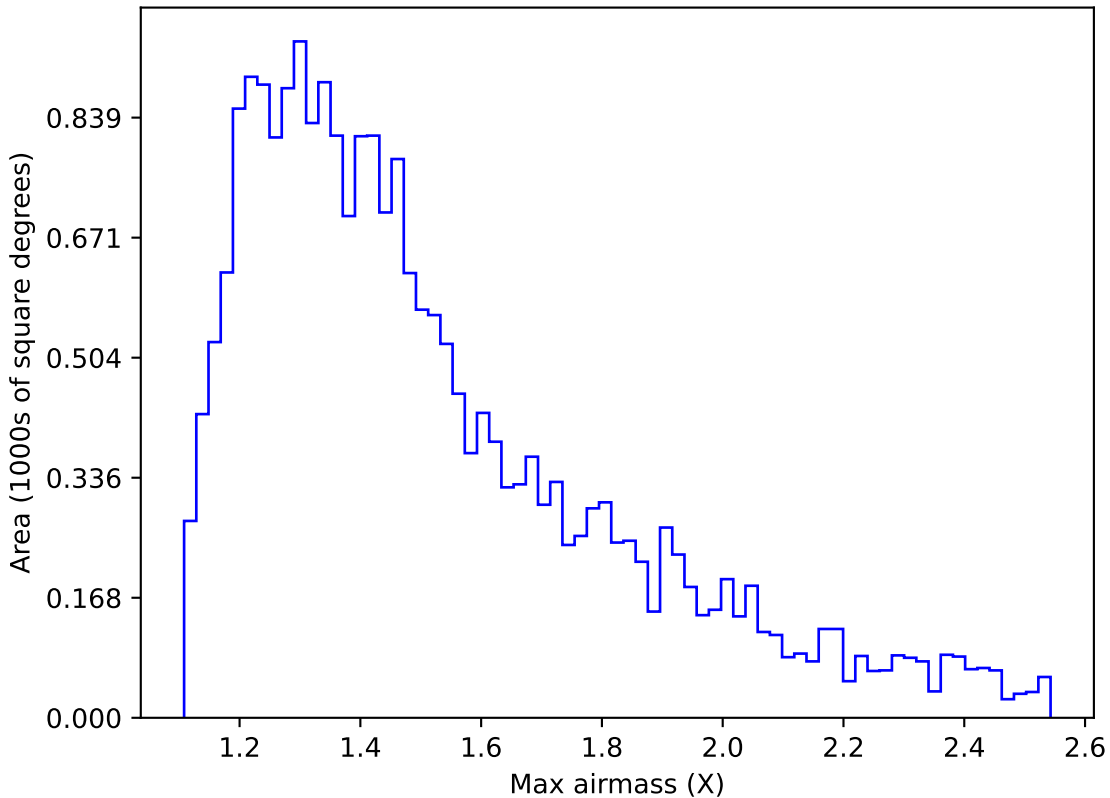
ddf_acor_sf10_lsf40_lsr20_v3.4_10yrs Yr 1 u band: Max airmass
