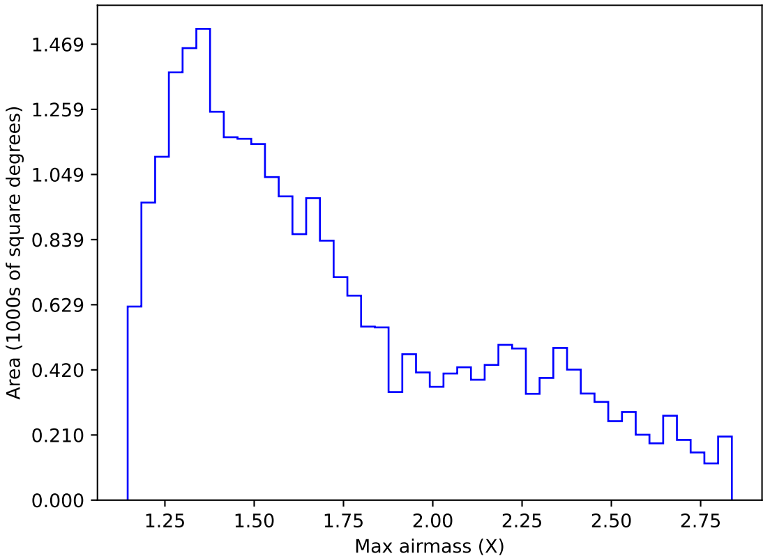
ddf_acor_sf10_lsf40_lsr20_v3.4_10yrs Yr 1 i band: Max airmass
