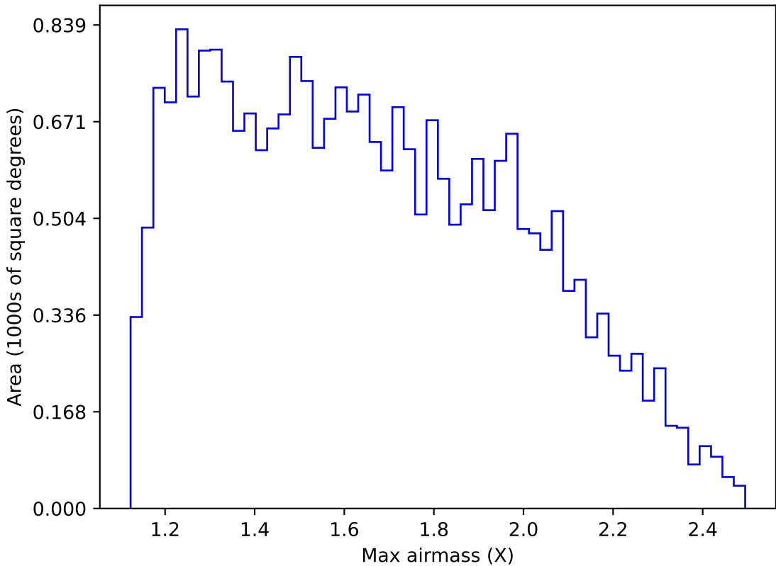
ddf_acor_sf10_lsf40_lsr20_v3.4_10yrs Yr 1 g band: Max airmass
