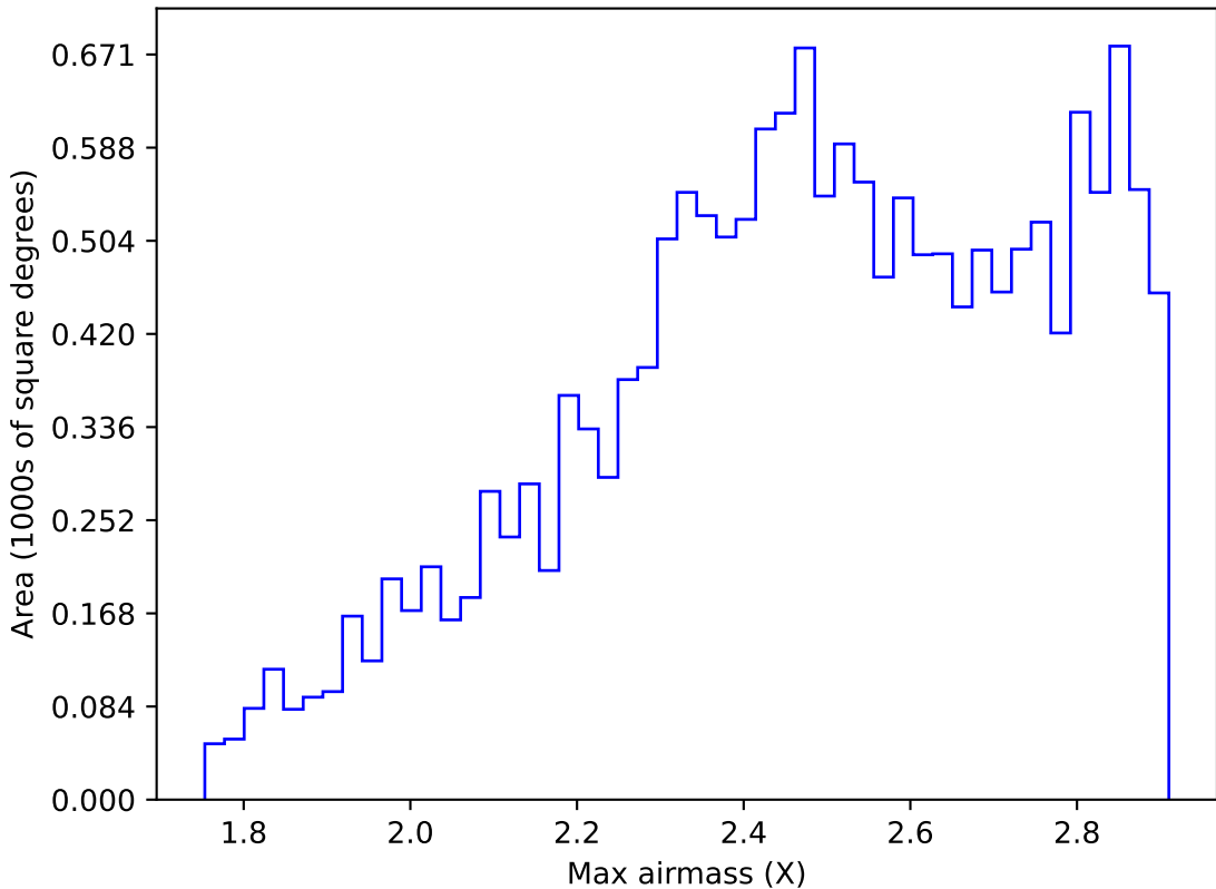
ddf_acor_sf10_lsf40_lsr20_v3.4_10yrs WFD z band: Max airmass
