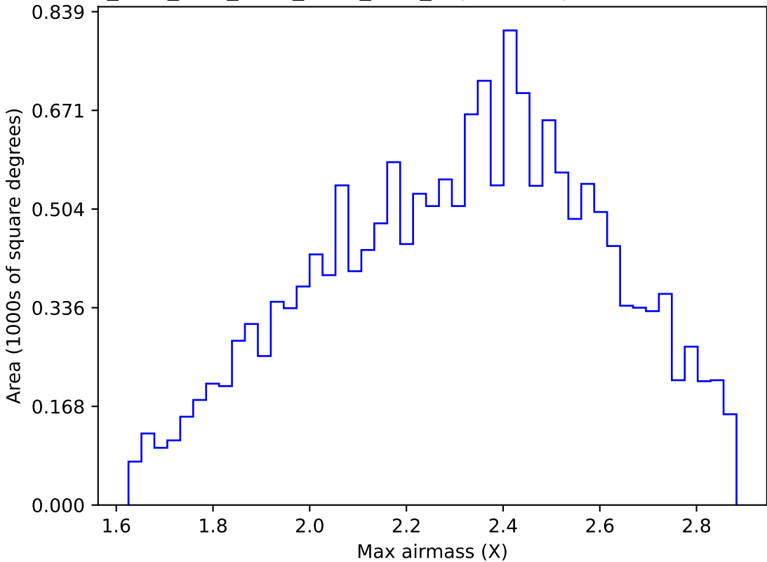
ddf_acor_sf10_lsf40_lsr20_v3.4_10yrs WFD y band: Max airmass
