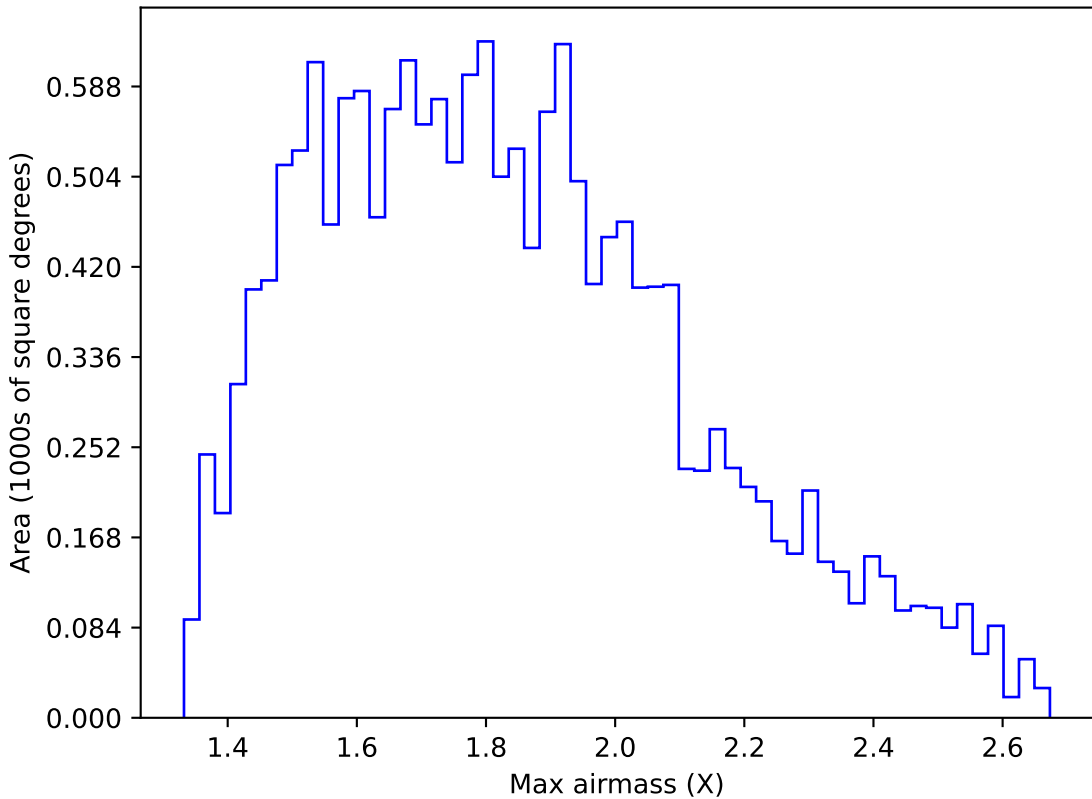
ddf_acor_sf10_lsf40_lsr20_v3.4_10yrs WFD u band: Max airmass
