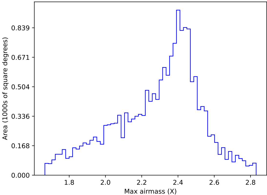
ddf_acor_sf10_lsf40_lsr20_v3.4_10yrs WFD r band: Max airmass
