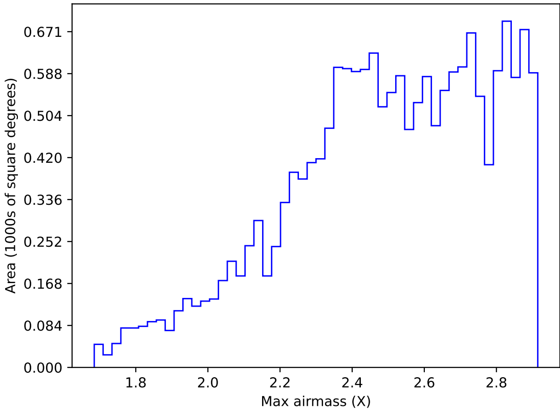
ddf_acor_sf10_lsf40_lsr20_v3.4_10yrs WFD i band: Max airmass
