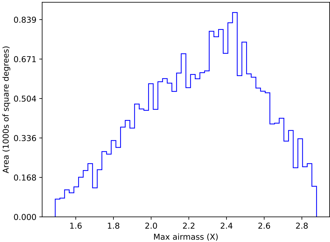
ddf_acor_sf10_lsf40_lsr20_v3.4_10yrs All sky y band: Max airmass
