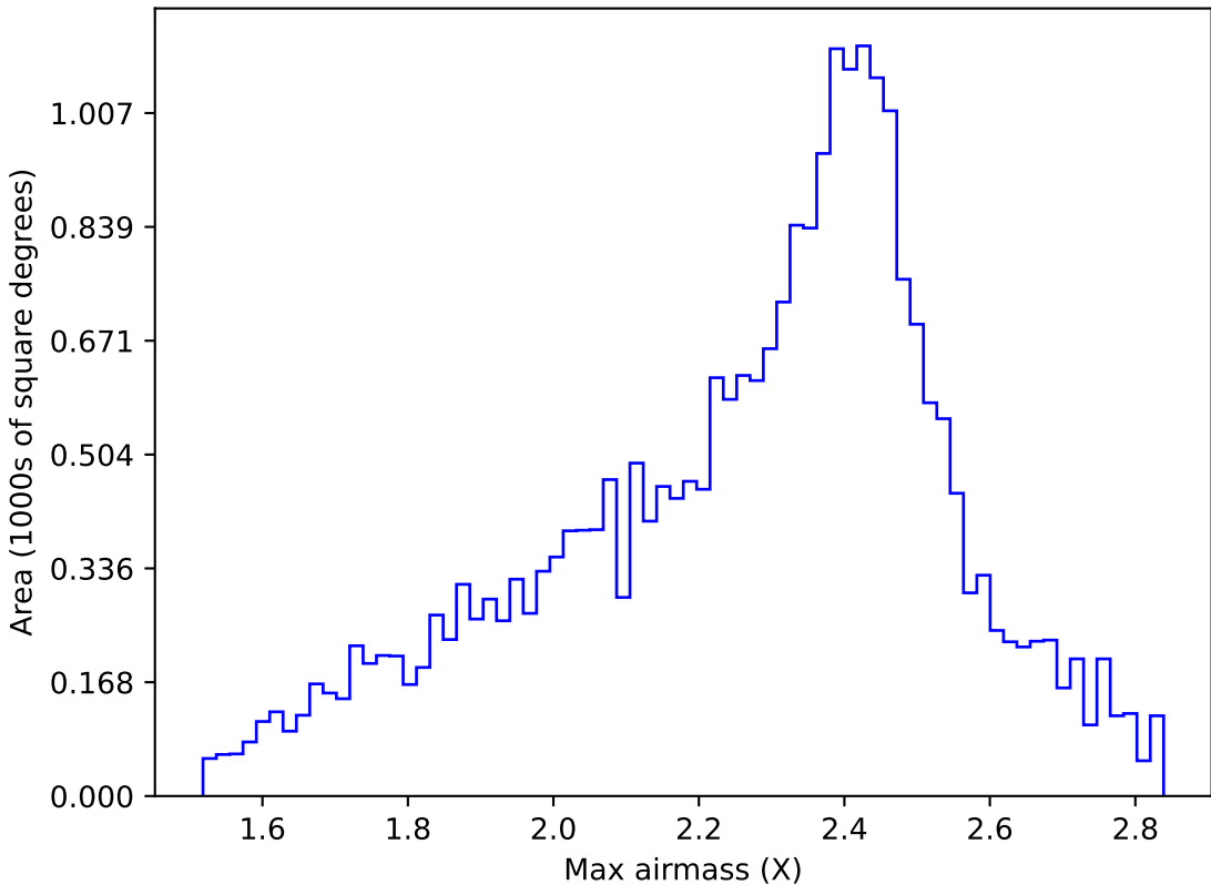
ddf_acor_sf10_lsf40_lsr20_v3.4_10yrs All sky r band: Max airmass
