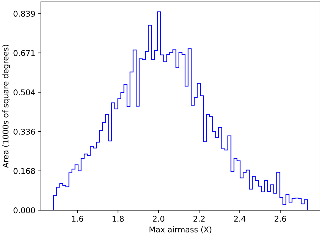
ddf_acor_sf10_lsf40_lsr20_v3.4_10yrs All sky g band: Max airmass
