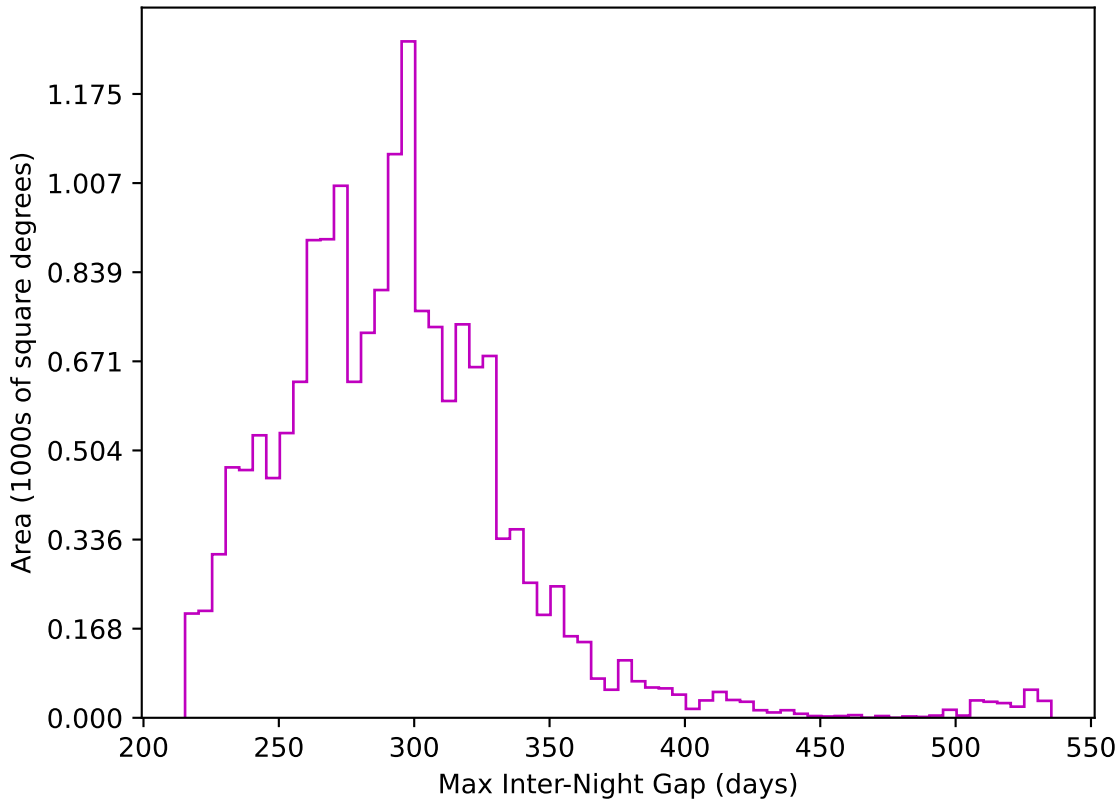
ddf_acor_sf10_lsf40_lsr20_v3.4_10yrs WFD z band: Max Inter-Night Gap
