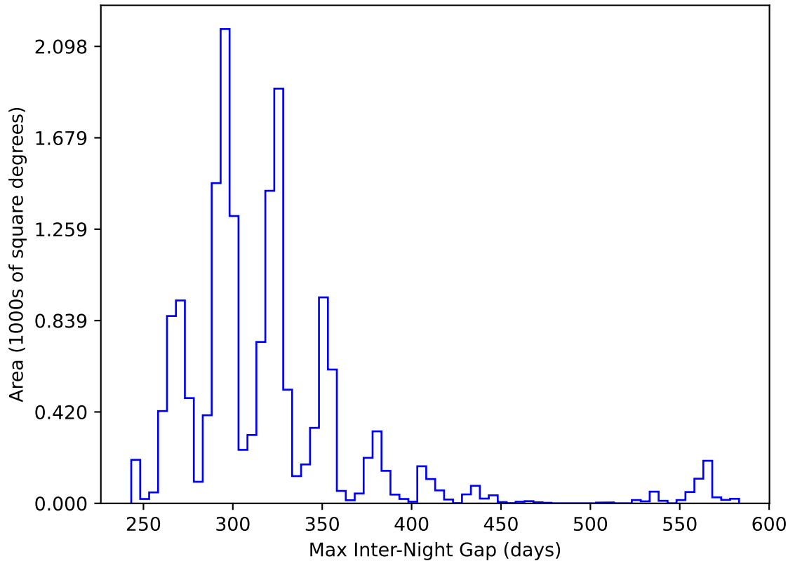
ddf_acor_sf10_lsf40_lsr20_v3.4_10yrs WFD y band: Max Inter-Night Gap
