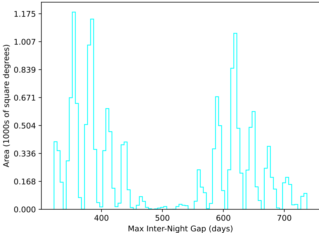
ddf_acor_sf10_lsf40_lsr20_v3.4_10yrs WFD u band: Max Inter-Night Gap
