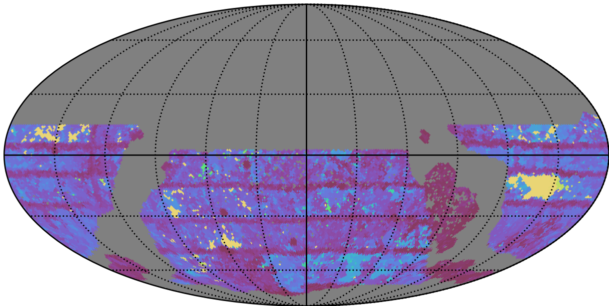
ddf_acor_sf10_lsf40_lsr20_v3.4_10yrs WFD r band: Max Inter-Night Gap
