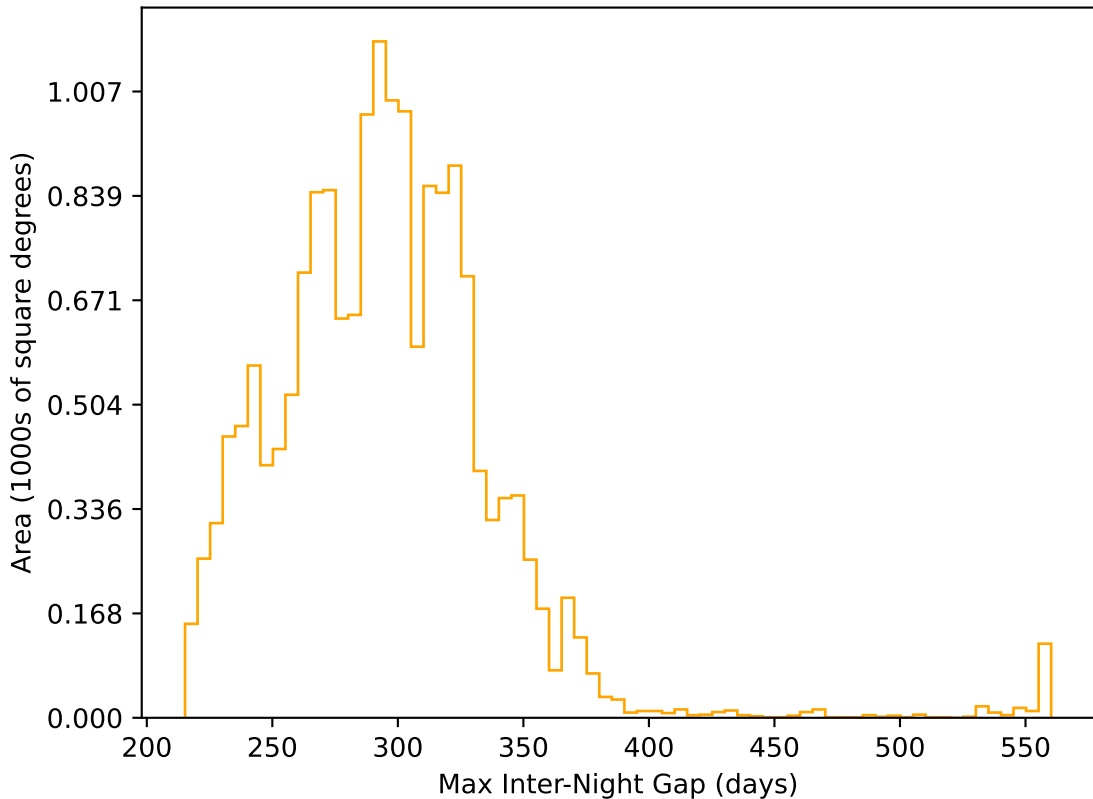
ddf_acor_sf10_lsf40_lsr20_v3.4_10yrs WFD r band: Max Inter-Night Gap
