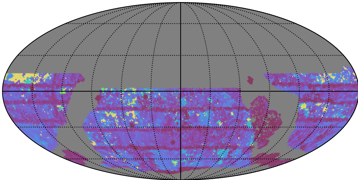
ddf_acor_sf10_lsf40_lsr20_v3.4_10yrs WFD i band: Max Inter-Night Gap
