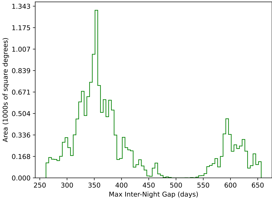
ddf_acor_sf10_lsf40_lsr20_v3.4_10yrs WFD g band: Max Inter-Night Gap
