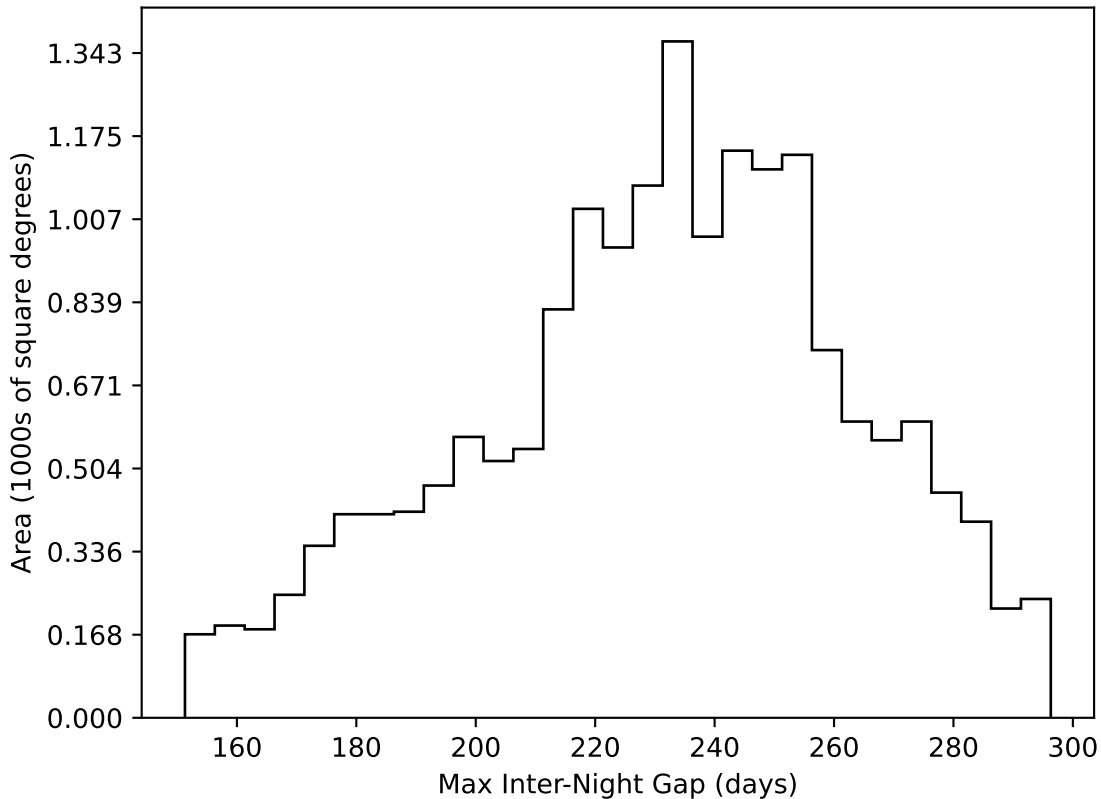
ddf_acor_sf10_lsf40_lsr20_v3.4_10yrs WFD all bands: Max Inter-Night Gap
