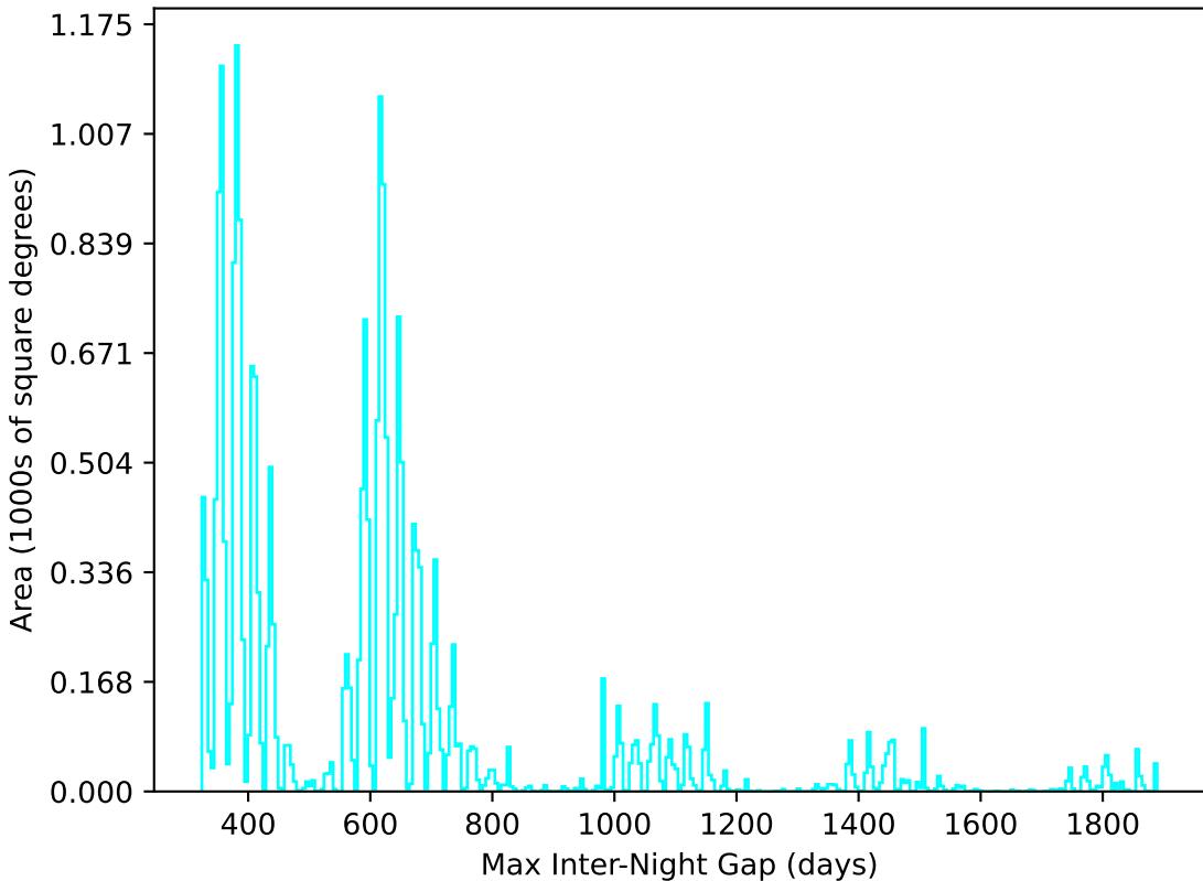
ddf_acor_sf10_lsf40_lsr20_v3.4_10yrs All sky u band: Max Inter-Night Gap
