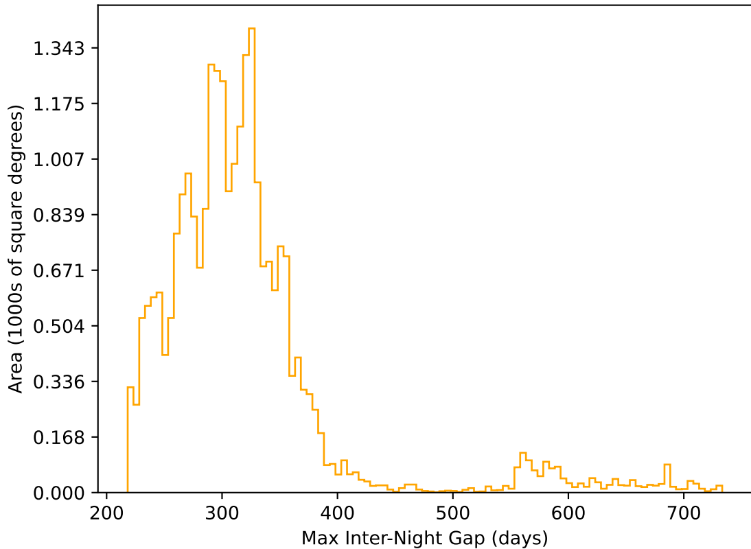
ddf_acor_sf10_lsf40_lsr20_v3.4_10yrs All sky r band: Max Inter-Night Gap
