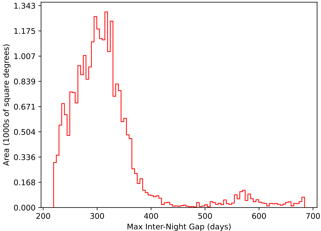
ddf_acor_sf10_lsf40_lsr20_v3.4_10yrs All sky i band: Max Inter-Night Gap
