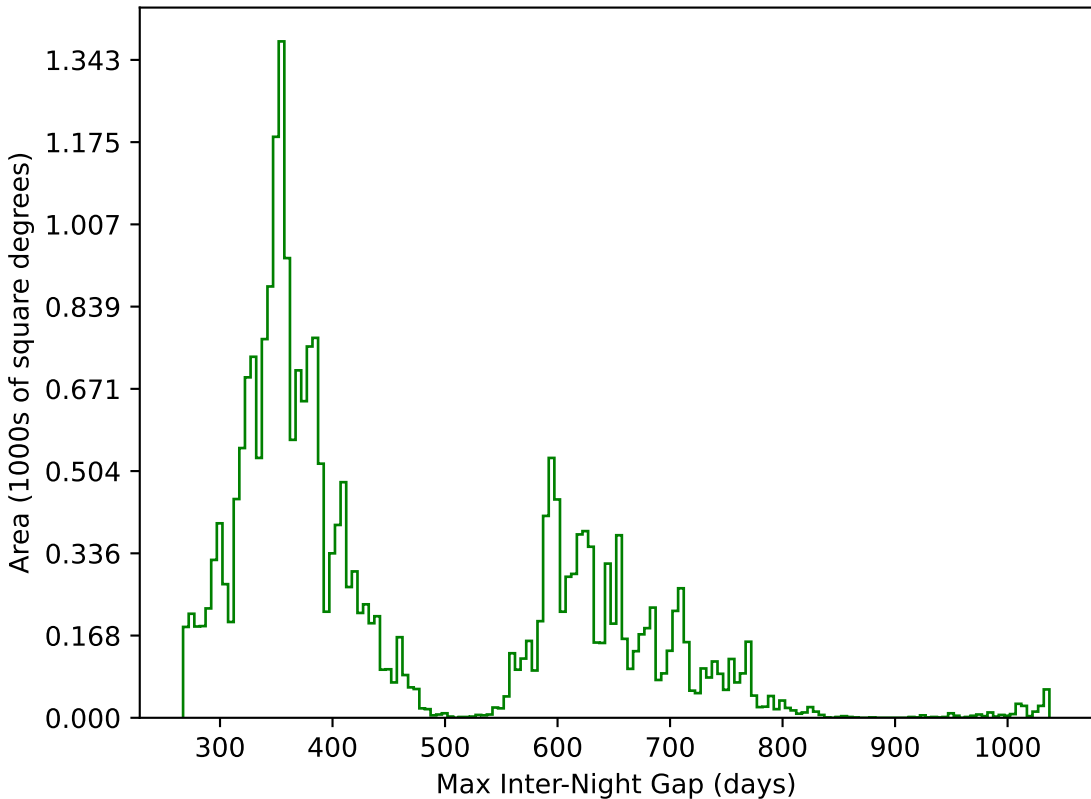
ddf_acor_sf10_ls40_lsr20_v3.4_10yrs All sky g band: Max Inter-Night Gap
