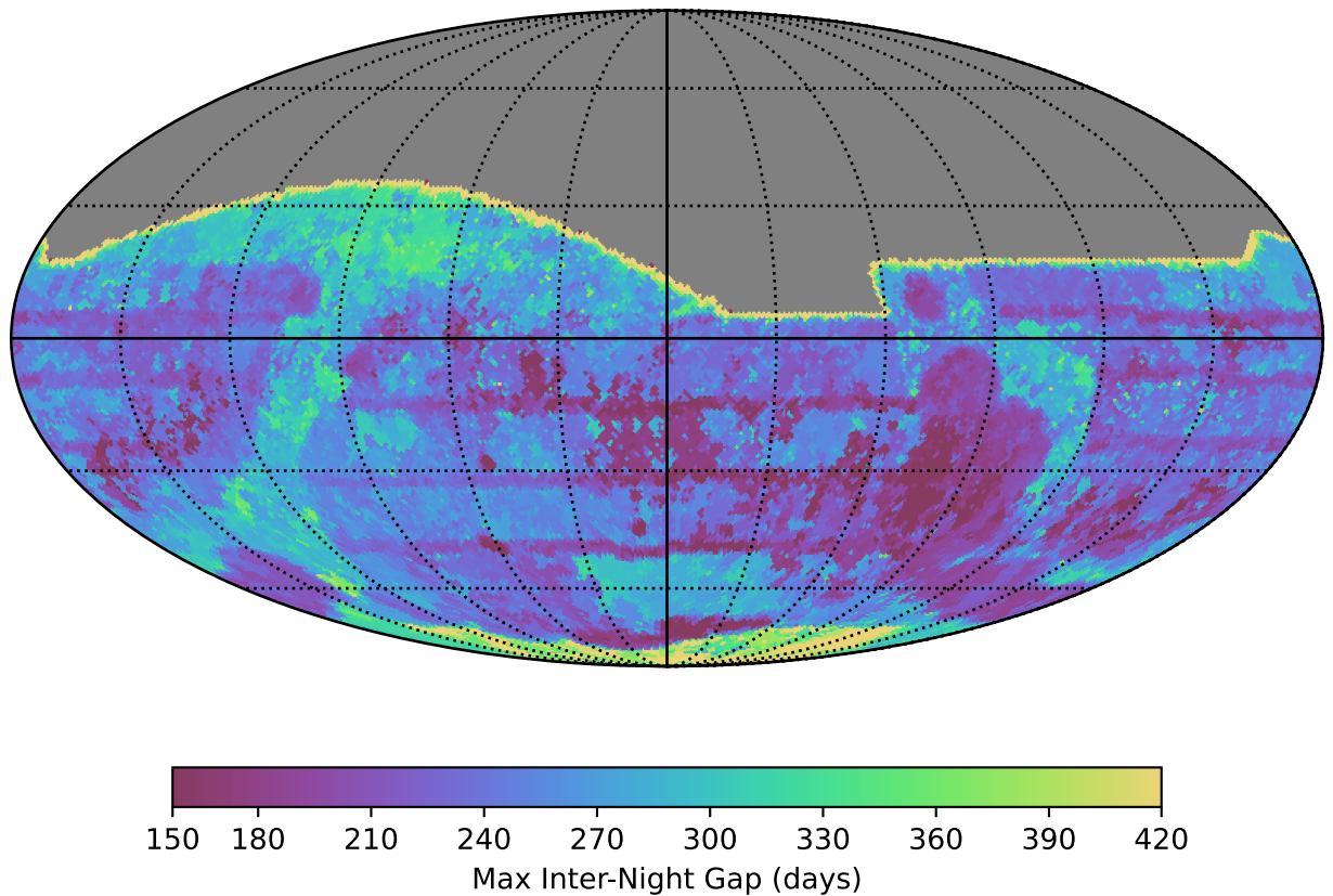
ddf_acor_sf10_lsf40_lsr20_v3.4_10yrs All sky all bands: Max Inter-Night Gap
