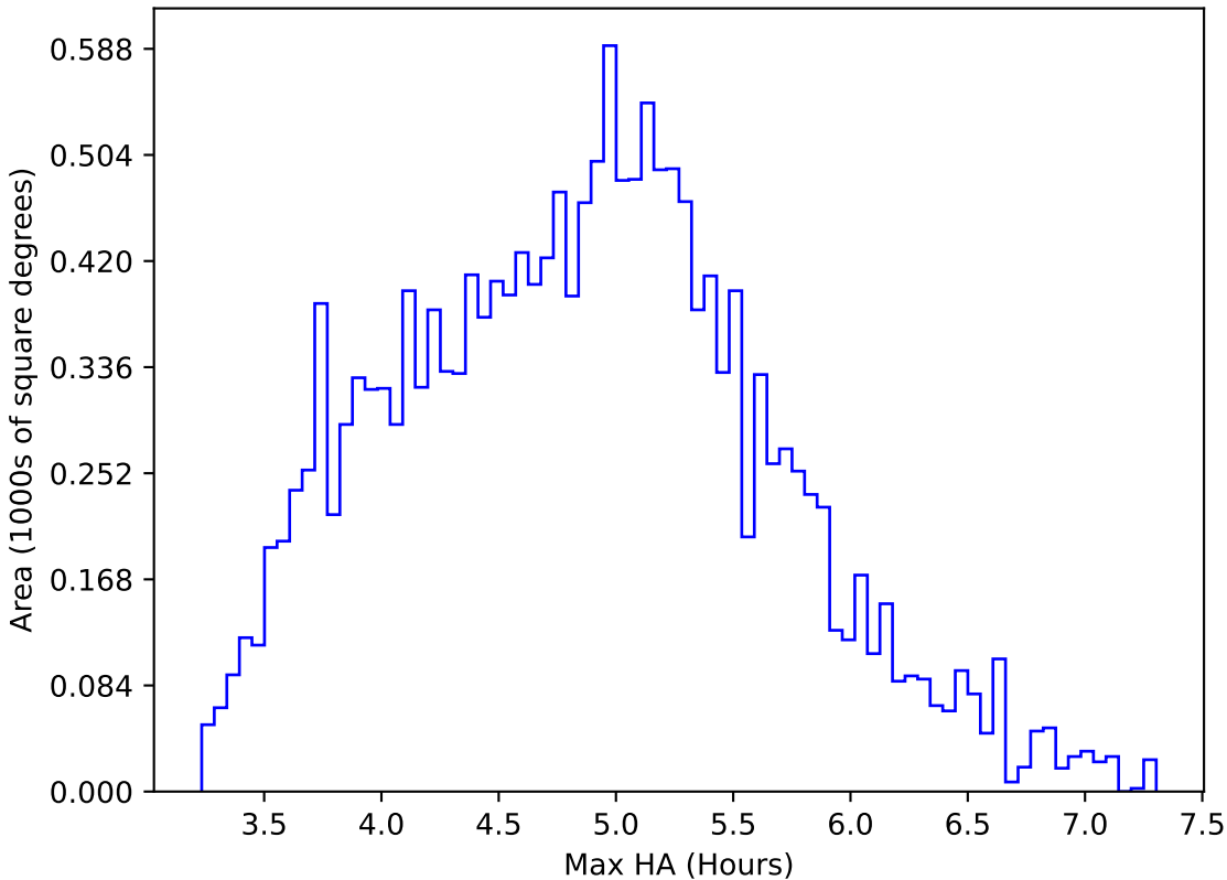
ddf_acor_sf10_lsf40_lsr20_v3.4_10yrs WFD z band: Max HA
