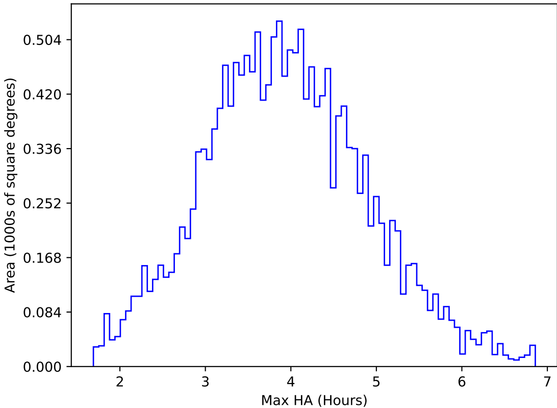
ddf_acor_sf10_lsf40_lsr20_v3.4_10yrs WFD u band: Max HA
