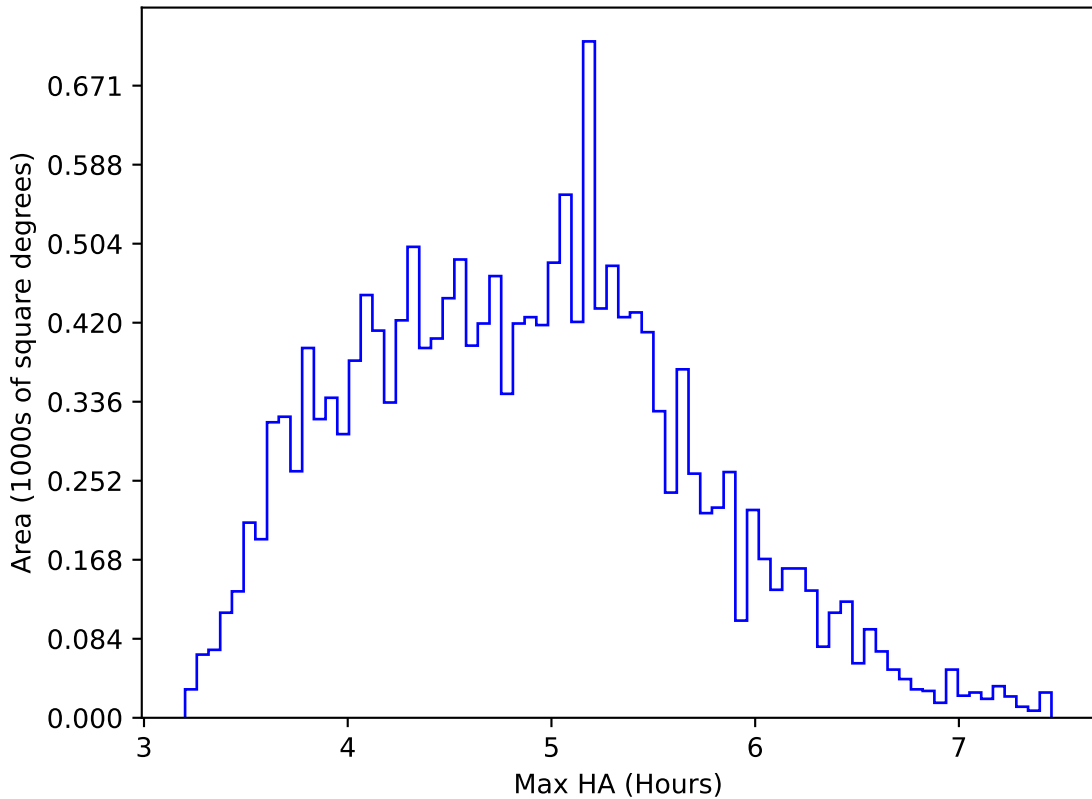
ddf_acor_sf10_lsf40_lsr20_v3.4_10yrs WFD i band: Max HA
