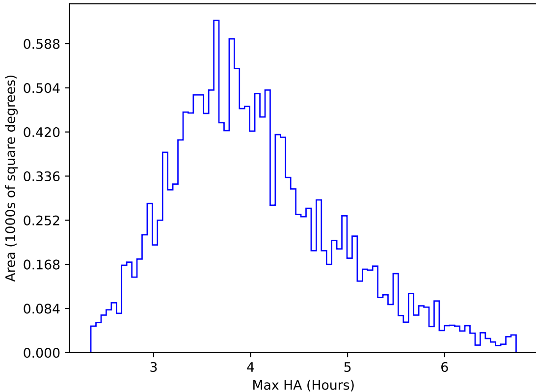
ddf_acor_sf10_lsf40_lsr20_v3.4_10yrs WFD g band: Max HA
