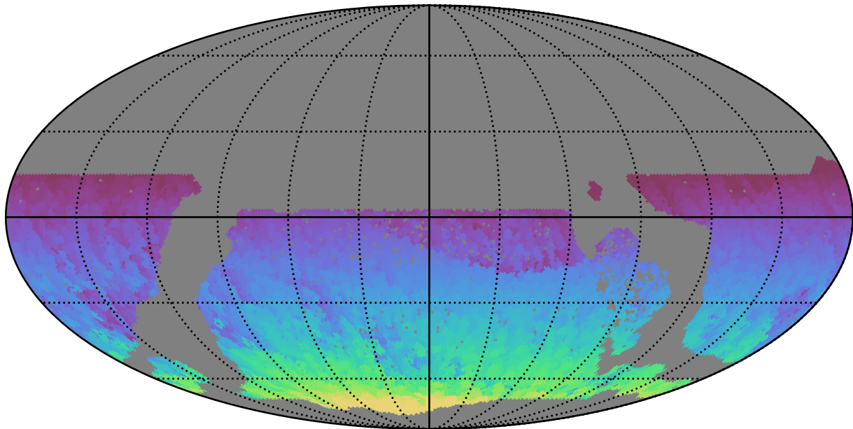
ddf_acor_sf10_lsf40_lsr20_v3.4_10yrs WFD all bands: Max HA
