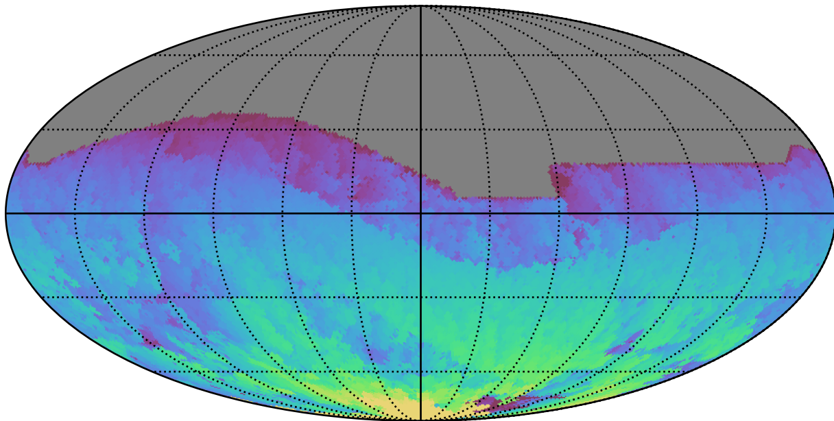
ddf_acor_sf10_lsf40_lsr20_v3.4_10yrs All sky z band: Max HA
