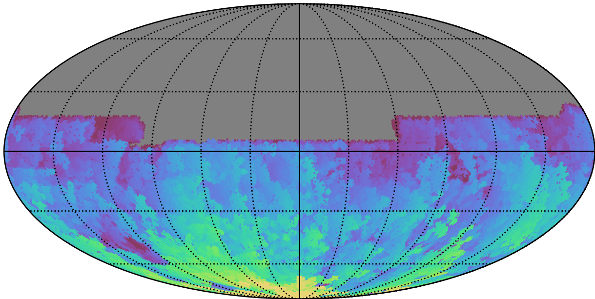
ddf_acor_sf10_lsf40_lsr20_v3.4_10yrs All sky u band: Max HA
