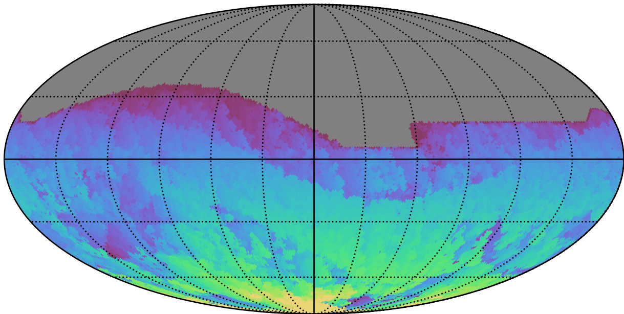
ddf_acor_sf10_lsf40_lsr20_v3.4_10yrs All sky i band: Max HA
