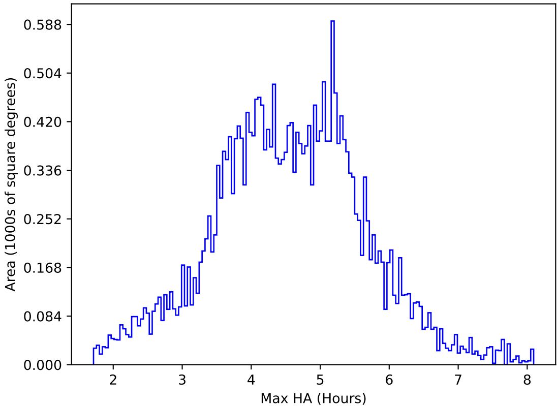
ddf_acor_sf10_lsf40_lsr20_v3.4_10yrs All sky i band: Max HA
