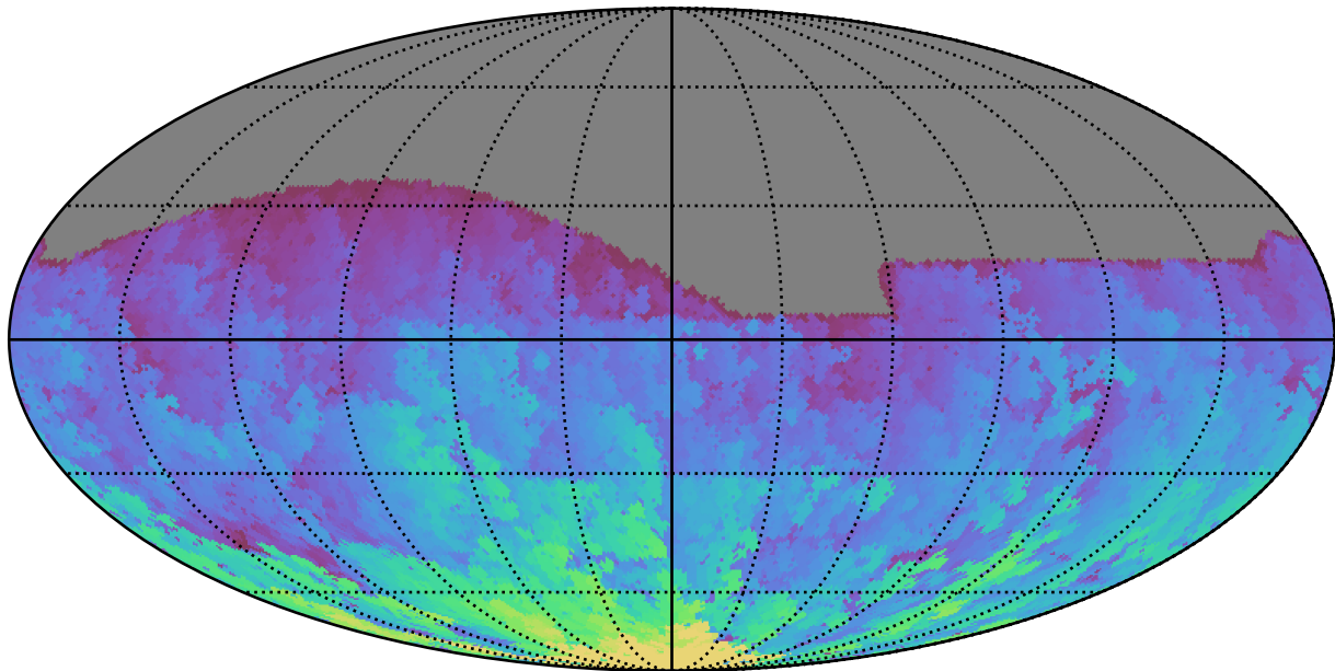
ddf_acor_sf10_lsf40_lsr20_v3.4_10yrs All sky g band: Max HA
