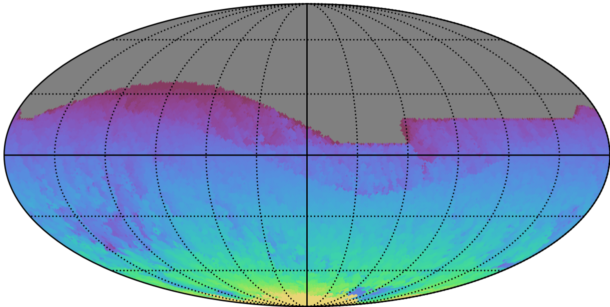
ddf_acor_sf10_lsf40_lsr20_v3.4_10yrs All sky all bands: Max HA
