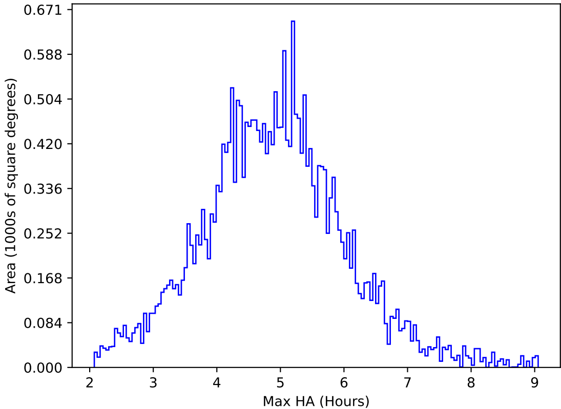
ddf_acor_sf10_lsf40_lsr20_v3.4_10yrs All sky all bands: Max HA
