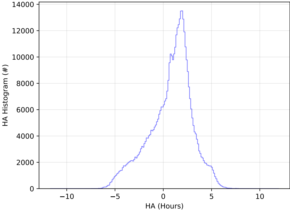
ddf_acor_sf10_lsf40_lsr20_v3.4_10yrs WFD z band: HA Histogram
