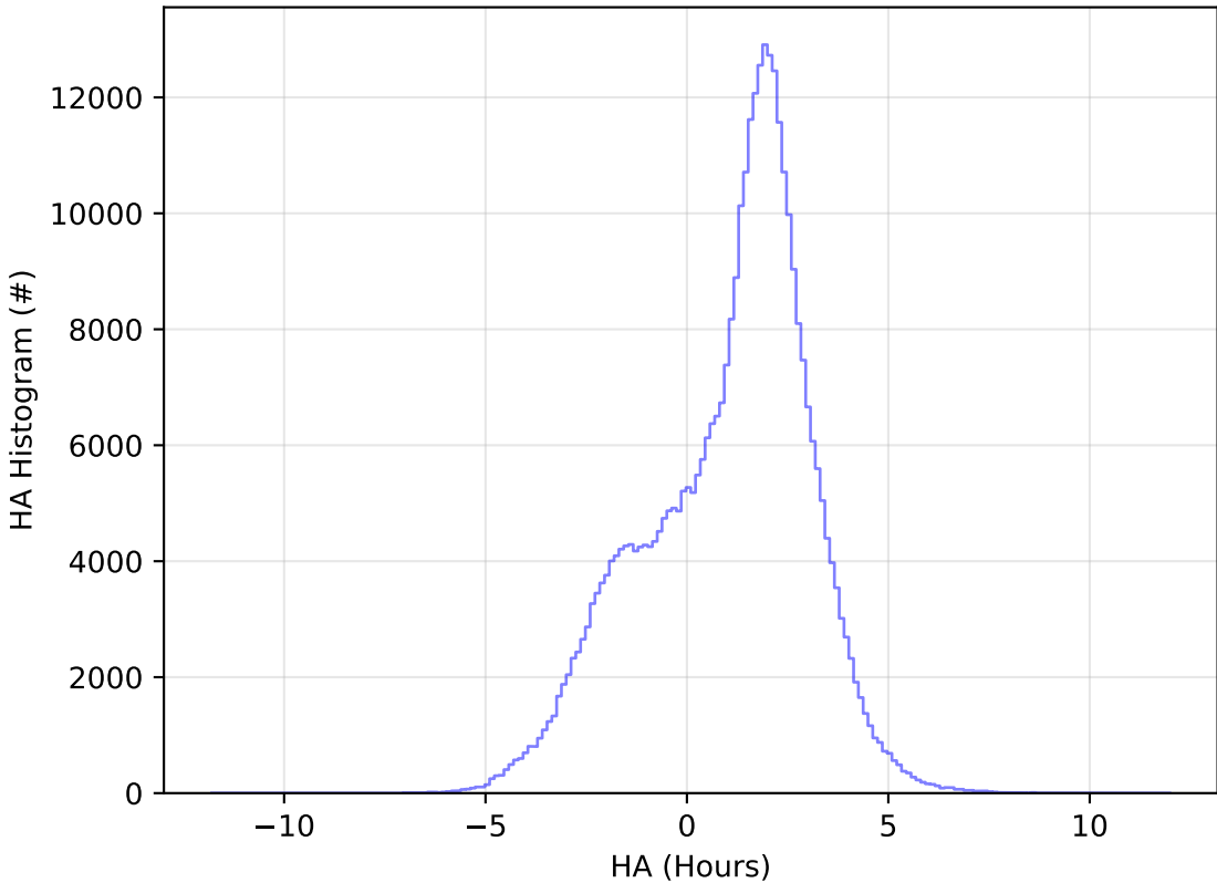
ddf_acor_sf10_ls40_lsr20_v3.4_10yrs WFD y band: HA Histogram
