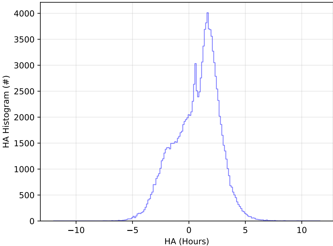
ddf_acor_sf10_lsf40_lsr20_v3.4_10yrs WFD u band: HA Histogram
