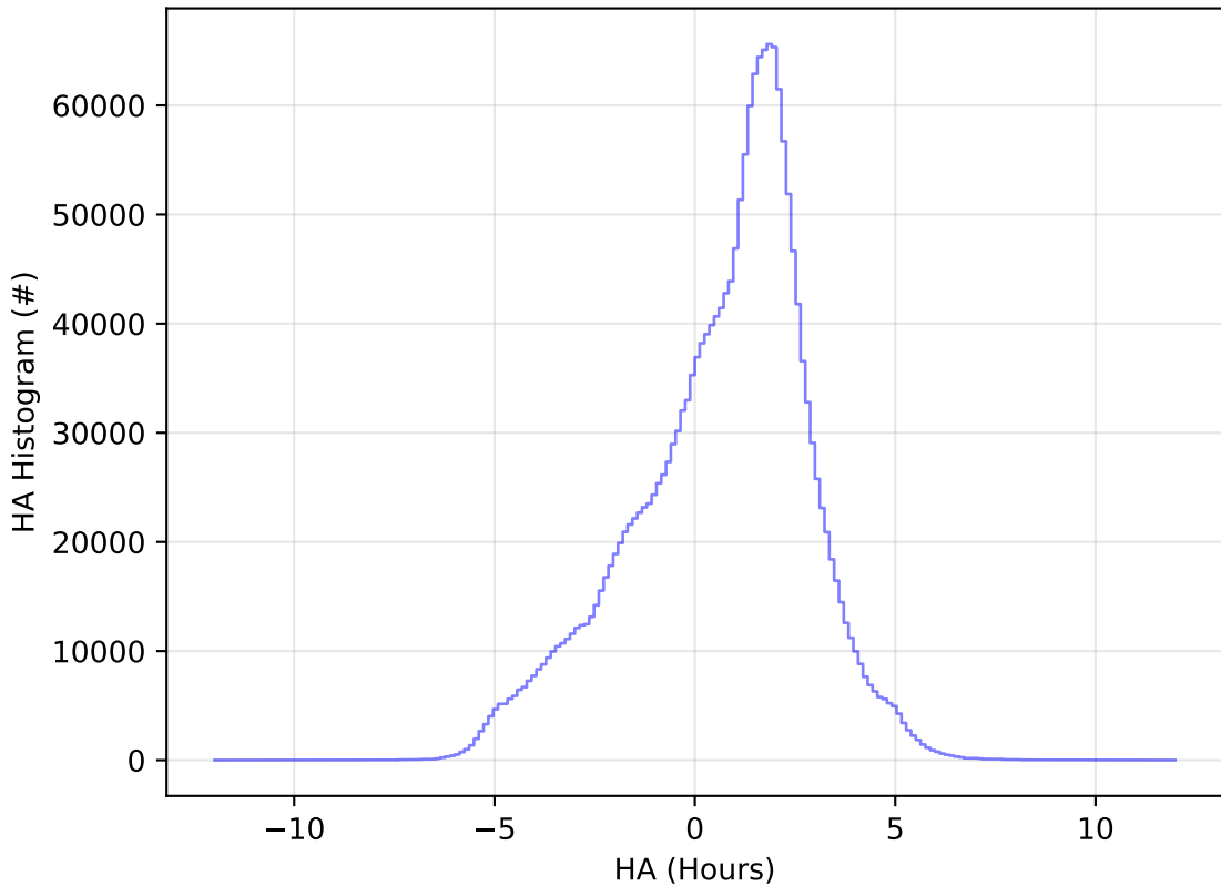
ddf_acor_sf10_lsf40_lsr20_v3.4_10yrs WFD all bands: HA Histogram
