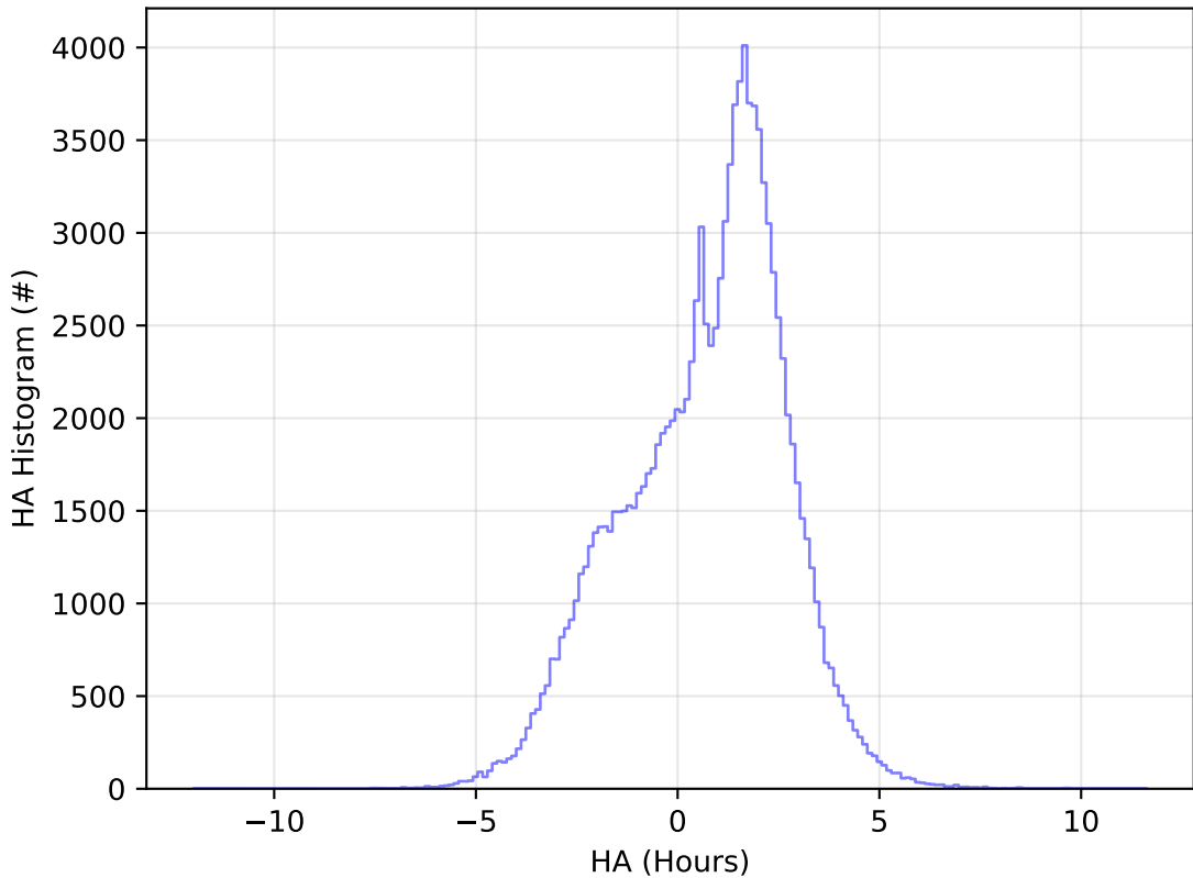
ddf_acor_sf10_lsf40_lsr20_v3.4_10yrs All sky u band: HA Histogram
