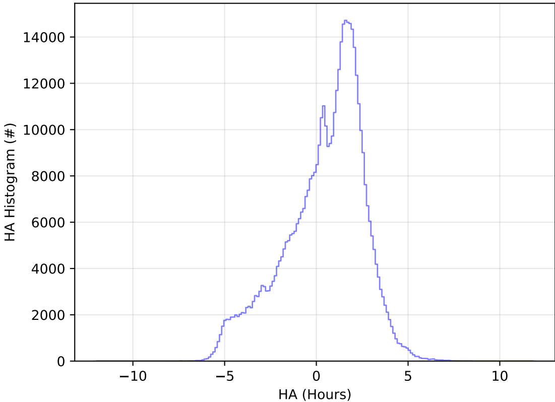
ddf_acor_sf10_lsf40_lsr20_v3.4_10yrs All sky r band: HA Histogram
