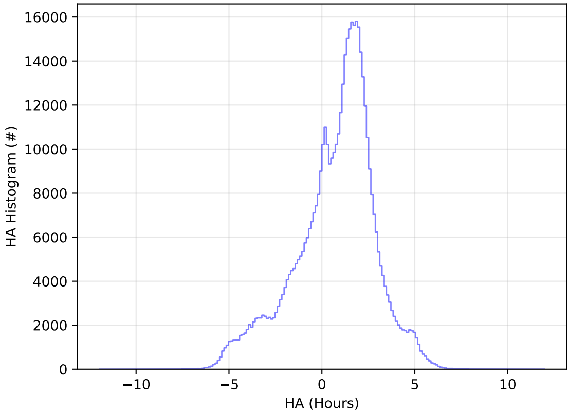
ddf_acor_sf10_lsf40_lsr20_v3.4_10yrs All sky i band: HA Histogram
