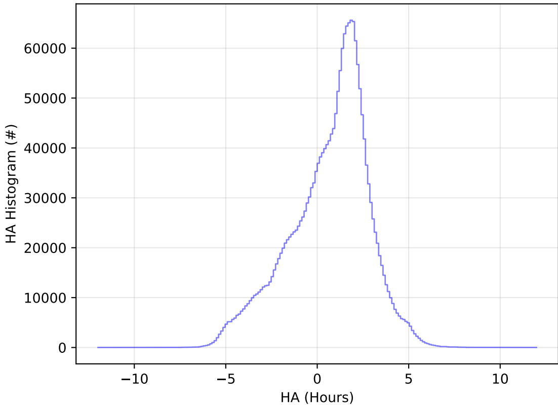
ddf_acor_sf10_lsf40_lsr20_v3.4_10yrs All sky all bands: HA Histogram
