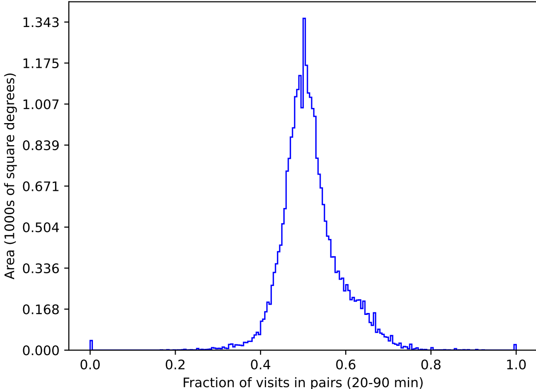
ddf_acor_sf10_lsf40_lsr20_v3.4_10yrs gri All sky: Fraction of visits in pairs (20-90 min)
