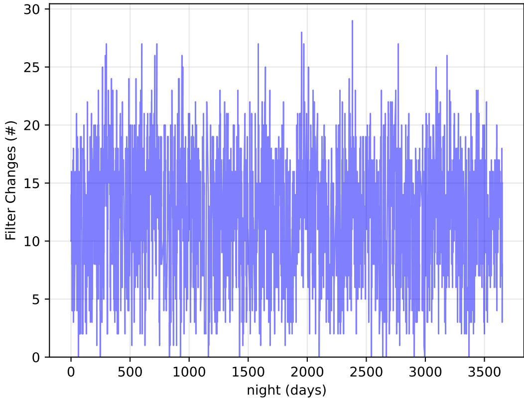
ddf_acor_sf10_lsf40_lsr20_v3.4_10yrs Per Night: Filter Changes
