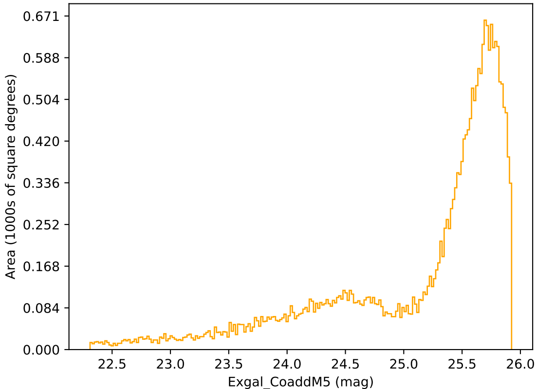
ddf_acor_sf10_lsf40_lsr20_v3.4_10yrs Yr 1 r band: Exgal_CoaddM5
