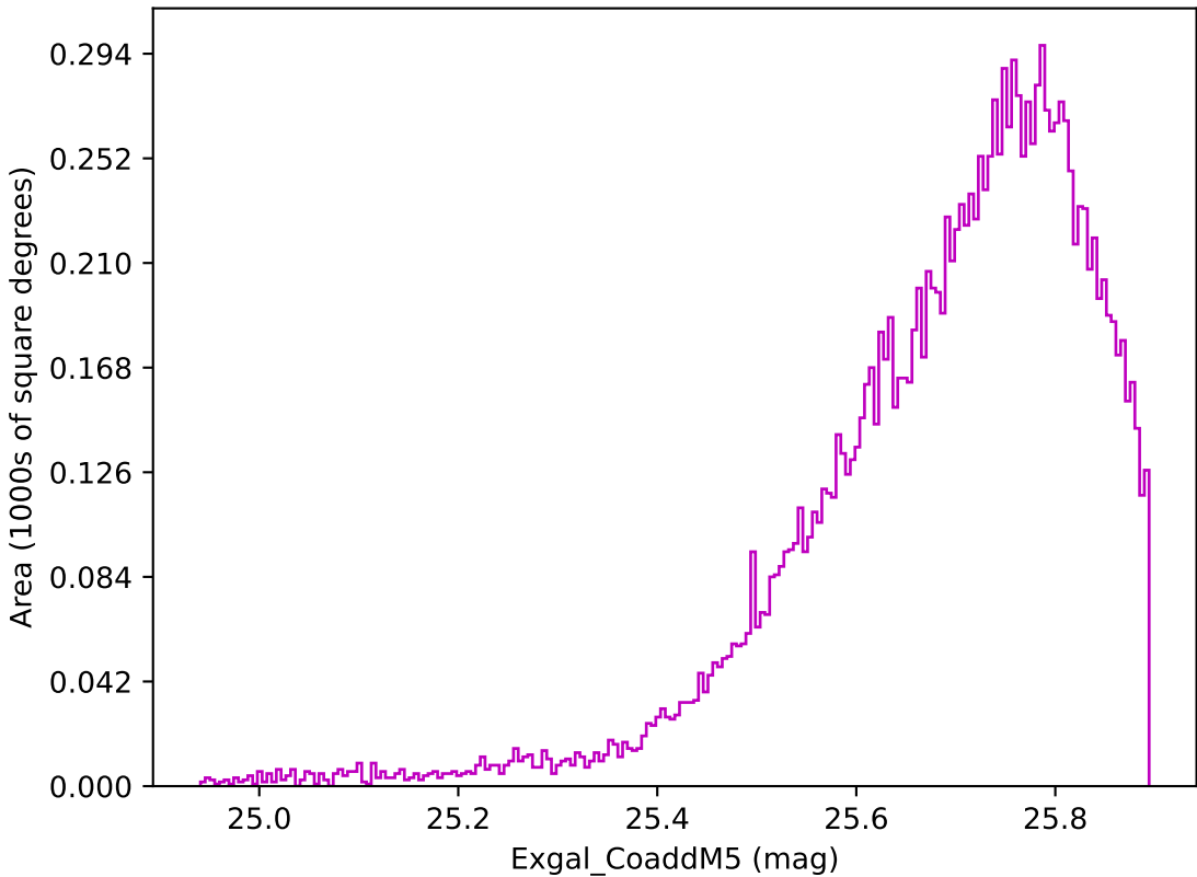
ddf_acor_sf10_lsf40_lsr20_v3.4_10yrs WFD z band: Exgal_CoaddM5
