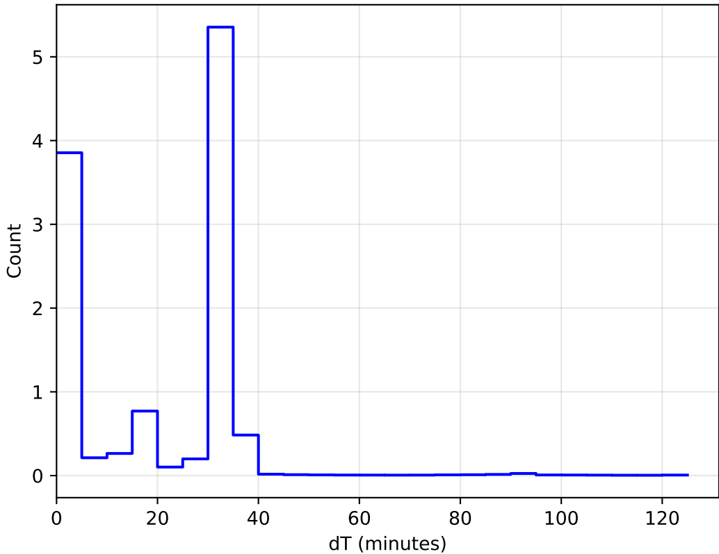
ddf_acor_sf10_lsf40_lsr20_v3.4_10yrs WFD: DeltaT Histogram 1e6
